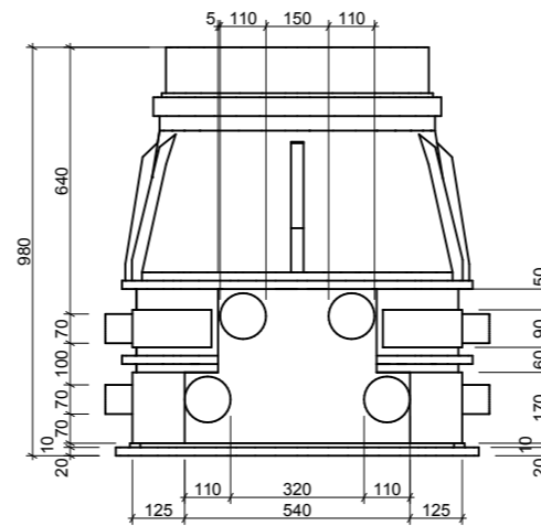
ELEVATION D
